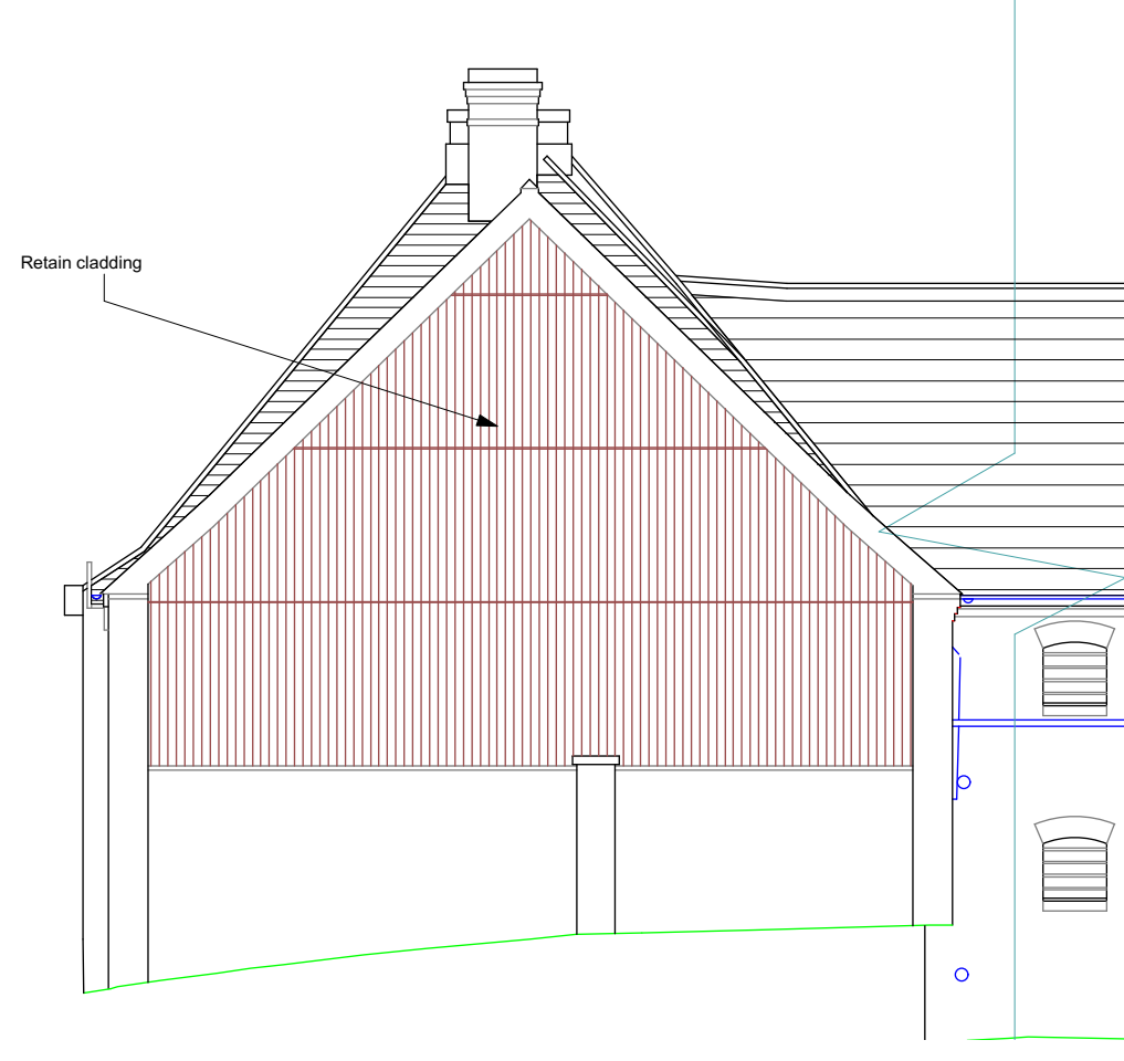
SIDE ELEVATION
