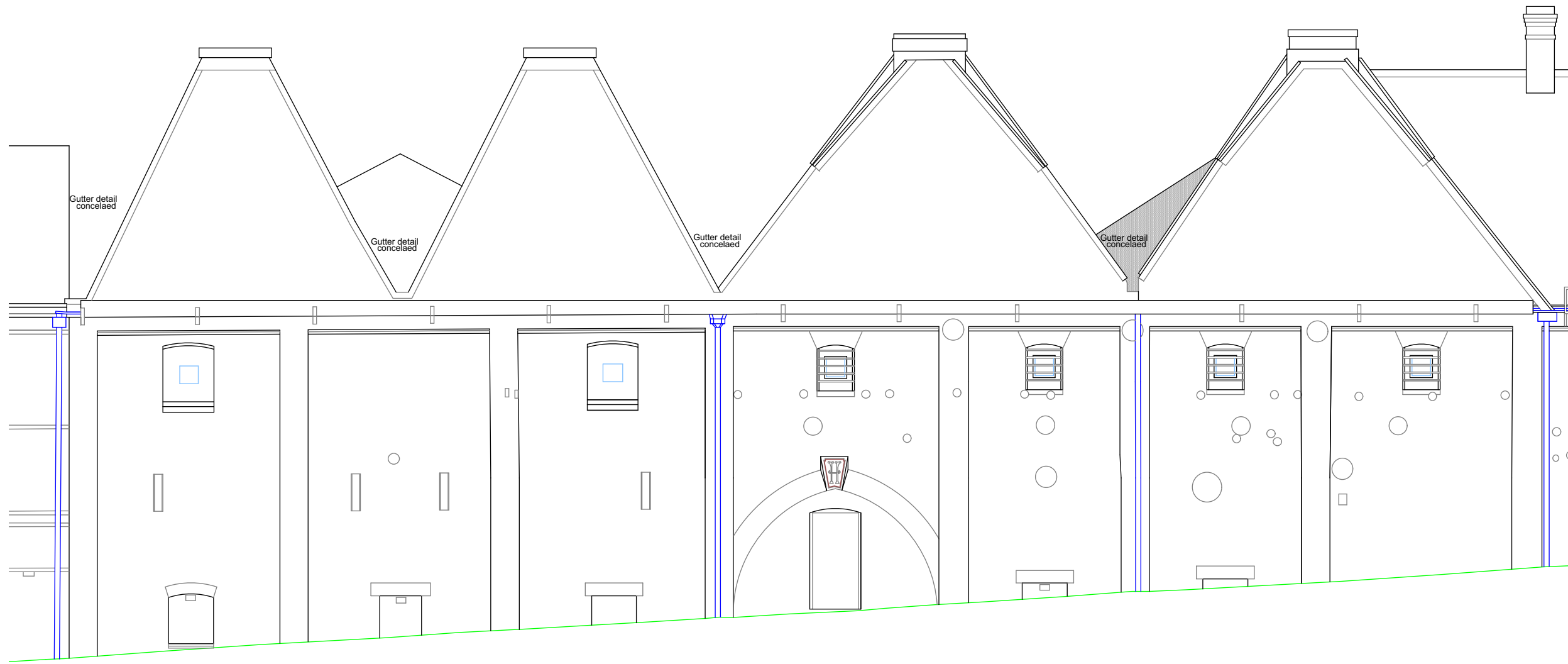
FRONT ELEVATION
