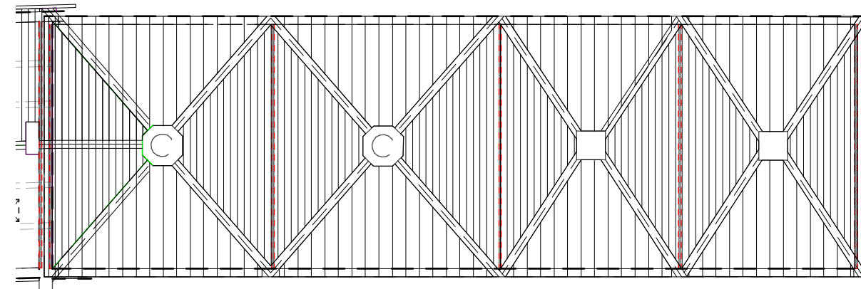
ROOF PLAN
